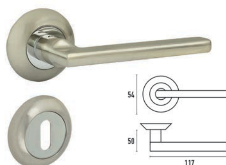
ALUMINIUM INTERNAL DOOR HANDLE WITH ROSETTE A1211, PAIR
