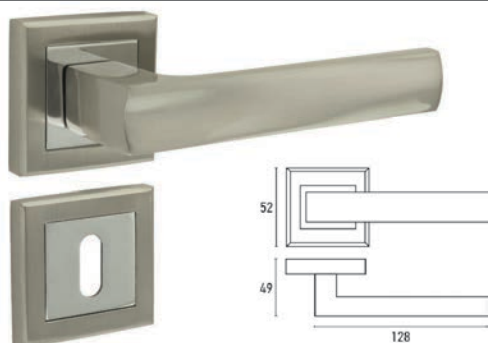
ALUMINIUM INTERNAL DOOR HANDLE WITH SQUARE ROSETTE A1453, PAIR
