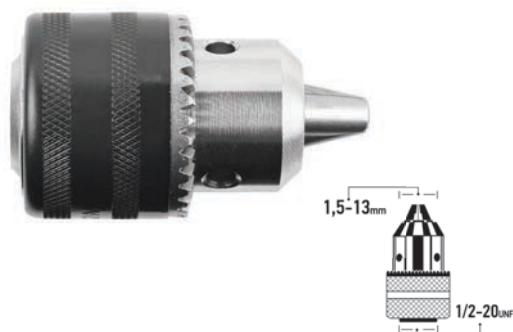
KEYED METALLIC DRILL CHUCK, 13mm - 1/2"
