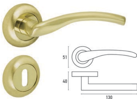
ALUMINIUM INTERNAL DOOR HANDLE WITH ROSETTE A1363, BRASS, PAIR
