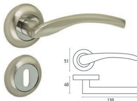
ALUMINIUM INTERNAL DOOR HANDLE WITH ROSETTE A1363, NICKEL, PAIR
