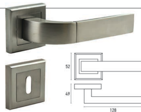
ALUMINIUM INTERNAL DOOR HANDLE WITH SQUARE ROSETTE A1432, PAIR
